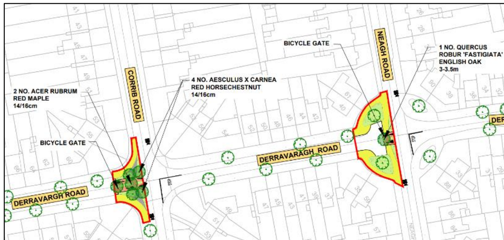
Figure 2-5-3: Proposed Road Closures at Derravaragh Road
