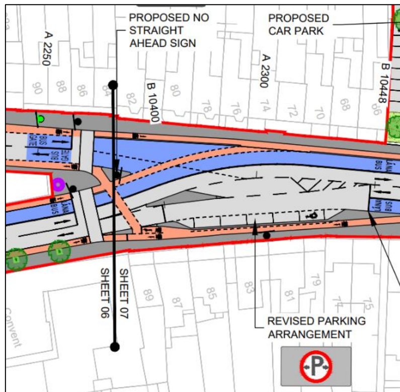
Figure 2-10-3: Junction of Kimmage Road Lower and Harold's Cross Road
