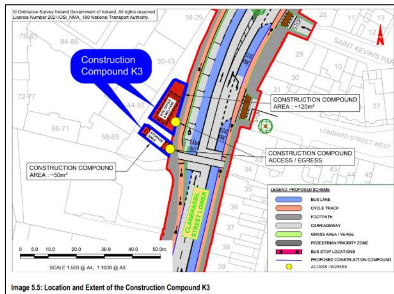
Figure 2-7-5: Construction Compound K3 at St. Patrick’s Court
