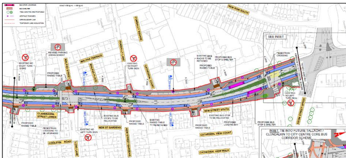
Figure 2-3-3: Extract from General Arrangement Drawings (Sheet 10)
