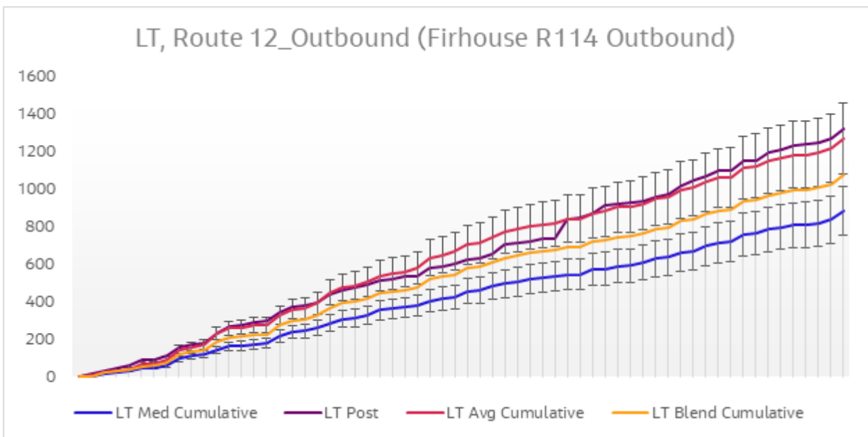
Diagram 6.17 Journey Time Validation Plot - Route 12 Outbound LT
