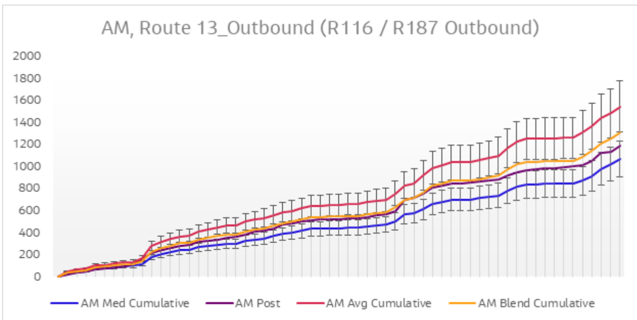
Diagram 6.15 Journey Time Validation Plot - Route 13 Outbound AM
