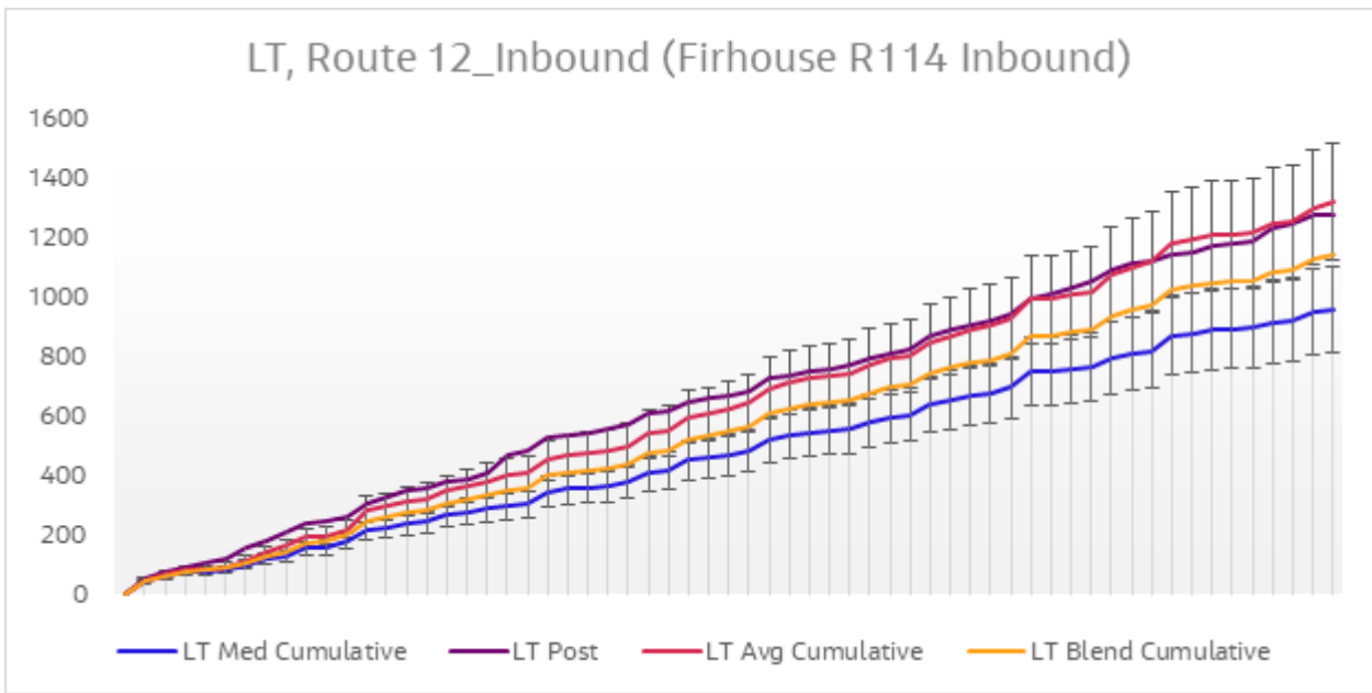
Diagram 6.16 Journey Time Validation Plot - Route 12 Inbound LT
