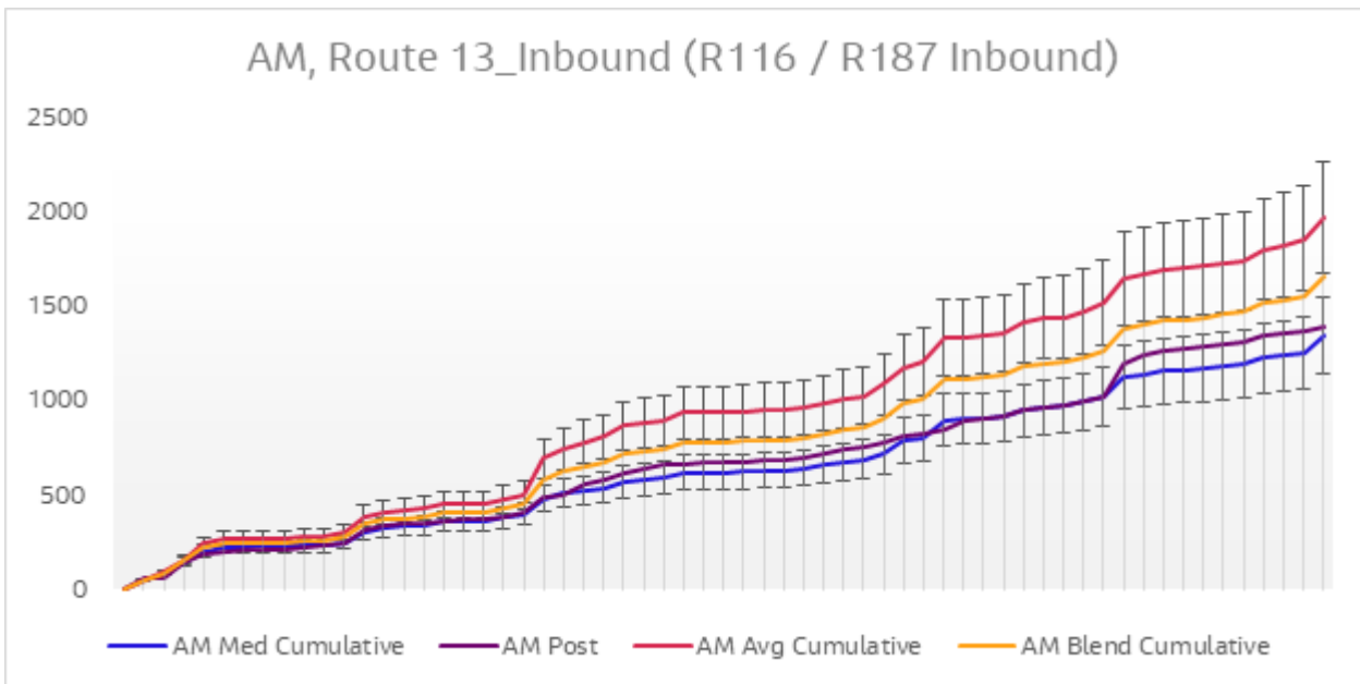
Diagram 6.14 Journey Time Validation Plot - Route 13 Inbound AM
