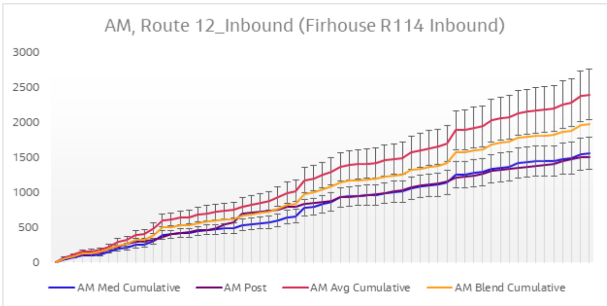
Diagram 6.12 Journey Time Validation Plot – Route 12 Inbound AM
