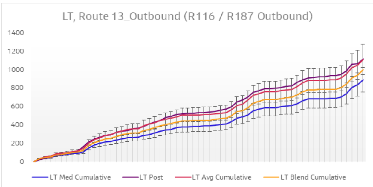
Diagram 6.19 Journey Time Validation Plot - Route 13 Outbound LT
