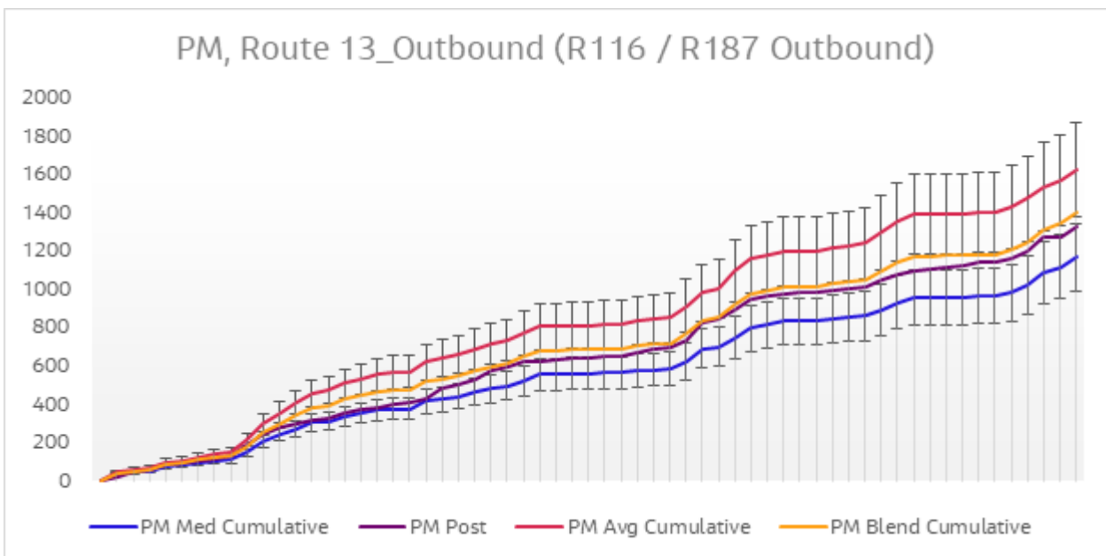
Diagram 6.27 Journey Time Validation Plot - Route 13 Outbound PM
