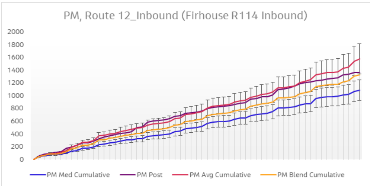
Diagram 6.24 Journey Time Validation Plot - Route 12 Inbound PM
