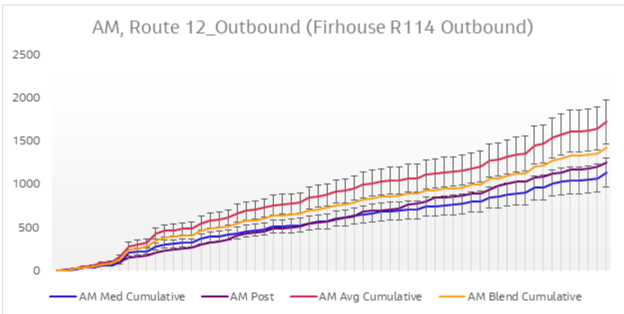
Diagram 6.13 Journey Time Validation Plot - Route 12 Outbound AM
