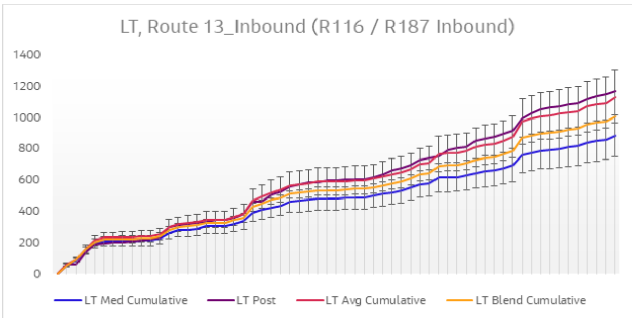
Diagram 6.18 Journey Time Validation Plot - Route 13 Inbound LT
