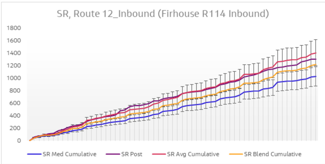
Diagram 6.20 Journey Time Validation Plot - Route 12 Inbound SR
